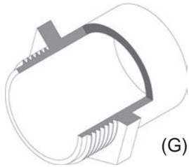
Nipple MP/MT
