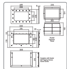
Liner Extension Throats – HD102LN
