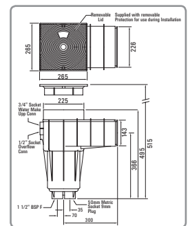
Concrete Weir Type – HD100SN Adjustable flow restrictor for bottom connection
