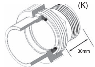
Socket Union P/MT
