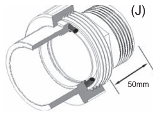
Socket Union P/MT
