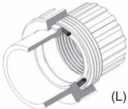
Socket Union P/FT
