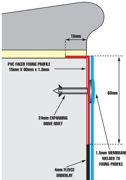
Side Mount PVC Profile
