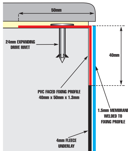
TOP Mount PVC Profile
