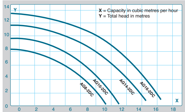
Performance Curve
