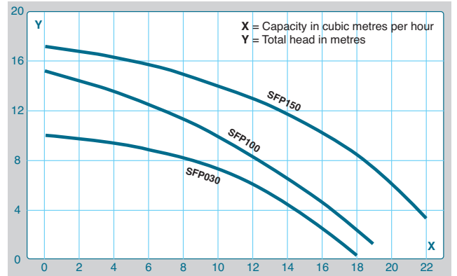
Performance Curve
