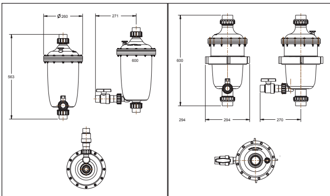
MC12
