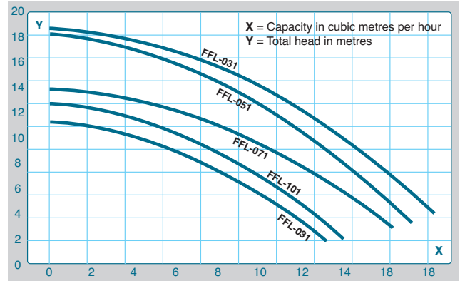
Performance Curve
