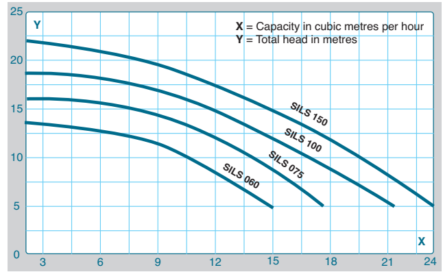
Performance Curve
